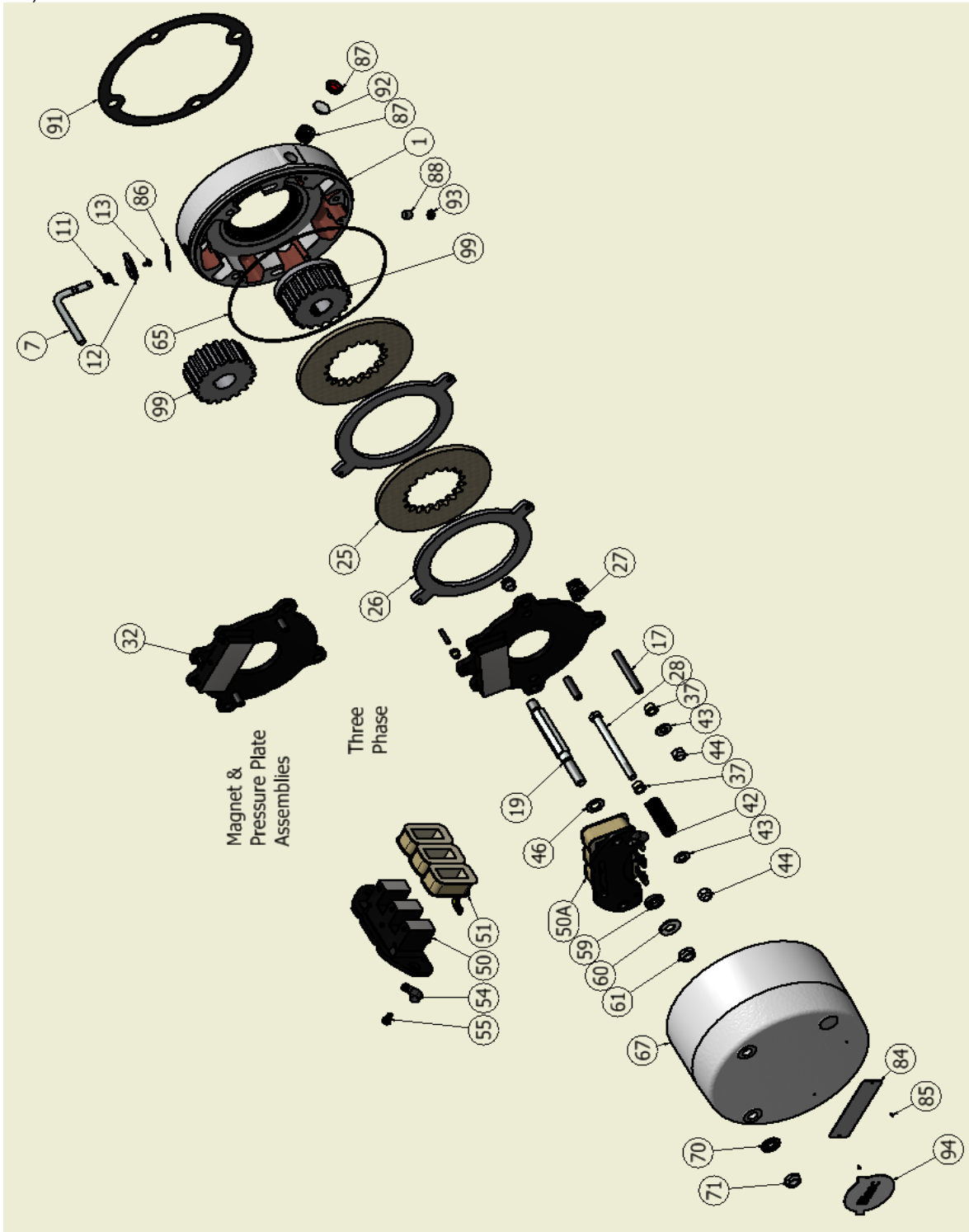
Figure 2 - Exploded View of Brake
