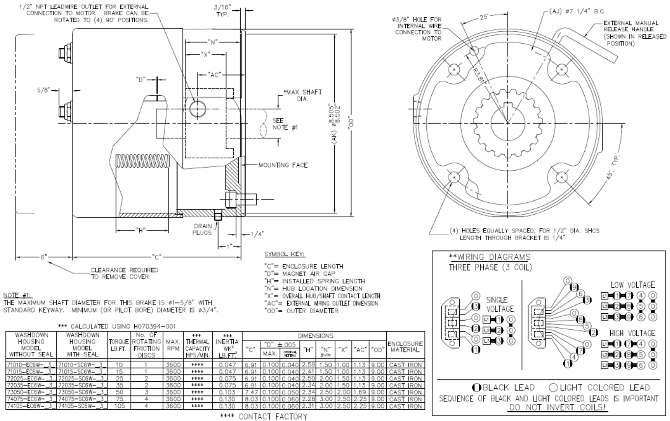
Figure.1 Brake Outline
