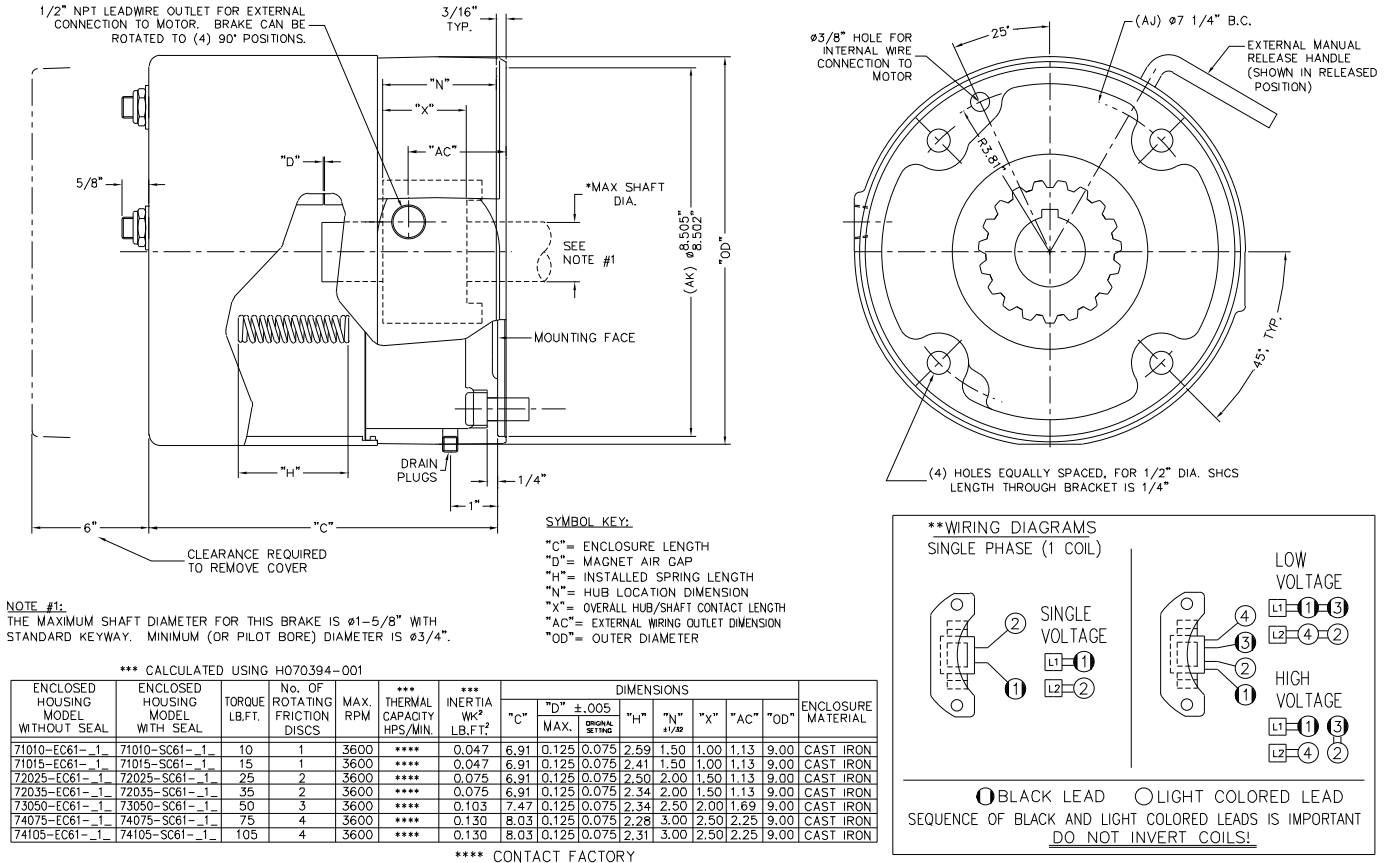
Figure.1 Brake Outline
